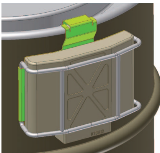
4 Conceptual mounting of prototype RFID tag on ES-3100 packaging: similar variations can be adopted for other drum types
