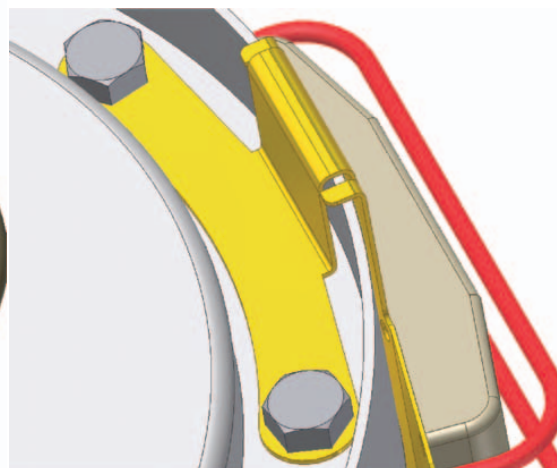
4 Conceptual mounting of prototype RFID tag on ES-3100 packaging: similar variations can be adopted for other drum types
